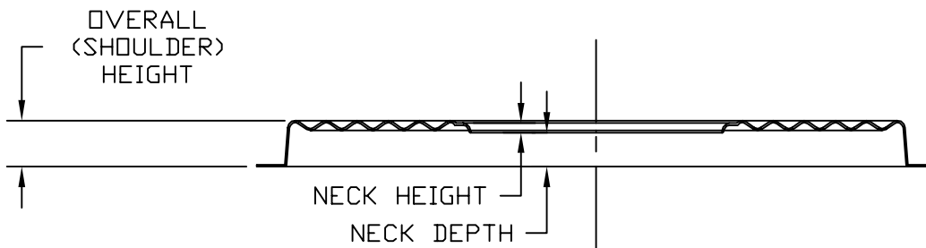
CUP SPIDER, NECK DOWN
