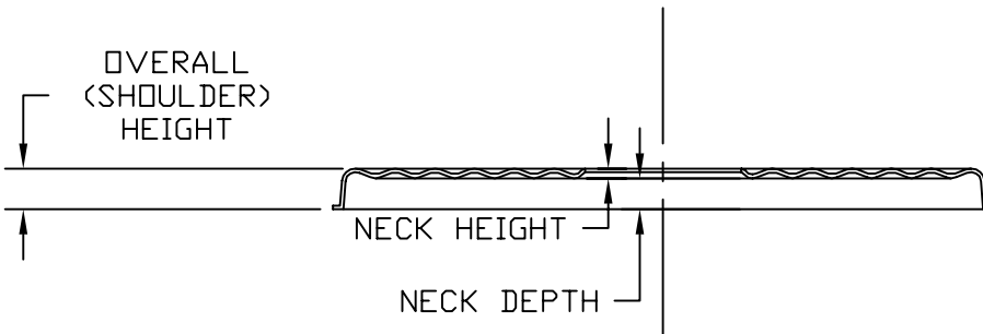
CUP SPIDER, NECK UP, EVEN WITH CORRUGATIONS (EWC)
